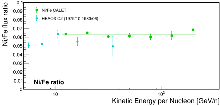
Figure 2: Nickel to iron flux ratio measured with CALET (green points). The errors bars are representative of statistical errors only. Data are fitted with a constant function giving \text{Ni/Fe} = 0.063 \pm 0.001 . Also plotted is the result from HEAO3-C2 [2].
