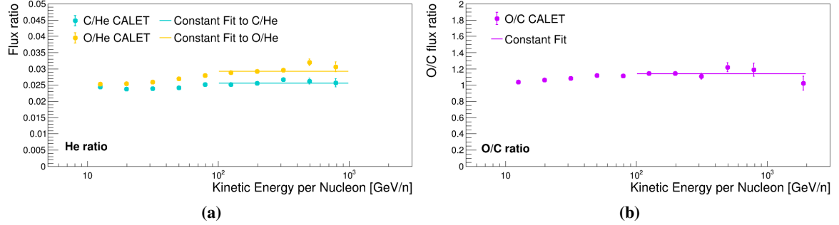
Figure 3: The flux ratios of light elements measured with CALET: (a) C/He (cyan fill circles) and O/He (yellow filled circles), (b) O/C (violet fill circles). The constant fit above 100 GeV/n is also reported (see the main text for the results).
