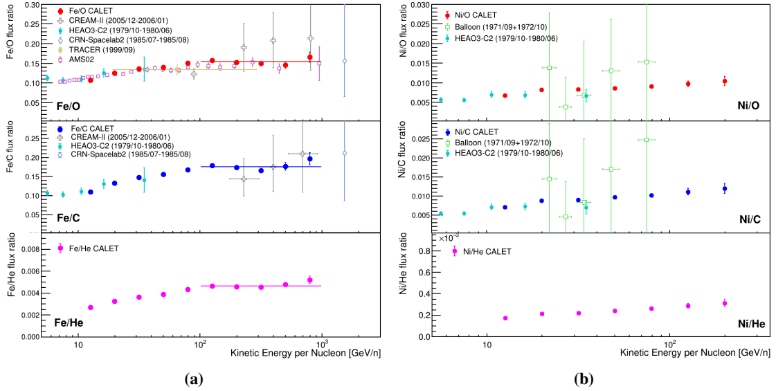
Figure 1: Measurement of the flux ratios (a) Fe/O, Fe/C and Fe/He and (b) Ni/O, Ni/C and Ni/He. CALET results are represented by the full colored circles and the error bars are representative of statistical uncertainty. In plot (a) the constant fit to the CALET results above 100 GeV/n is reported (see the main text for the results). Also plotted the measurement from HEAO3-C2 (cyan full squares), CREAM-II (gray open crosses), TRACER (mustard full squares), CRN (lilac open diamonds), HEN (green open squares).
