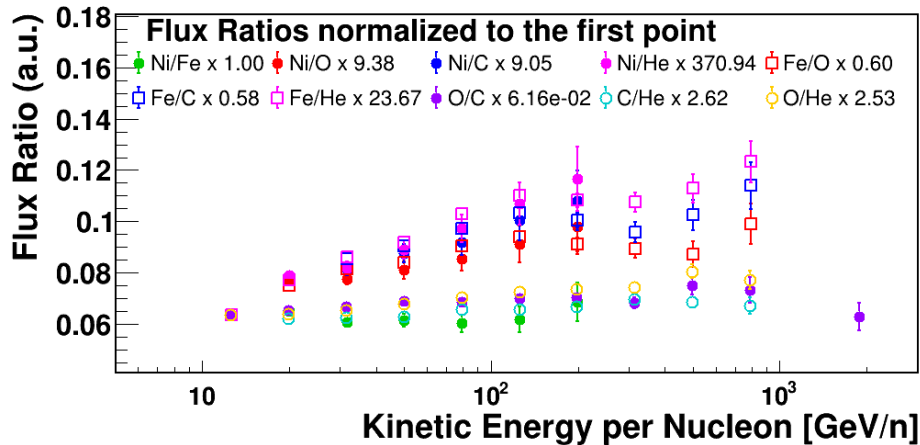
Figure 4: Comparison of CALET flux ratios: Ni/O (red points), Ni/C (blue points), Ni/He (magenta points), Fe/O (red squares), Fe/C (blue squares), Fe/He (magenta squares), O/C (violet points), C/He (cyan points) and O/He (yellow points) are normalized to the first point of Ni/Fe (green points).
